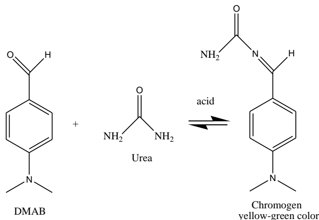
Fig. 3. Schem of DMAB-urea reaction.
